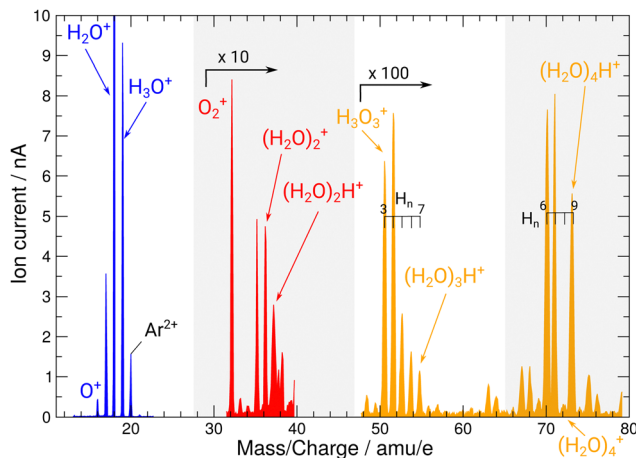
Fig. 2 Mass spectrum of ion beams from the FLAGS in the regions featuring the relevant cationic species and protonated water clusters. The mass spectrum was produced using the cluster setting of the ion source (third column in Table 1). For clusters containing three and four oxygen atoms, a variety of clusters with a different number of H atoms are produced. Mass ranges with no water cluster signal ( 22\text{--}30 \text{ u e}^{-1} and 38\text{--}48 \text{ u e}^{-1} ) are omitted.
