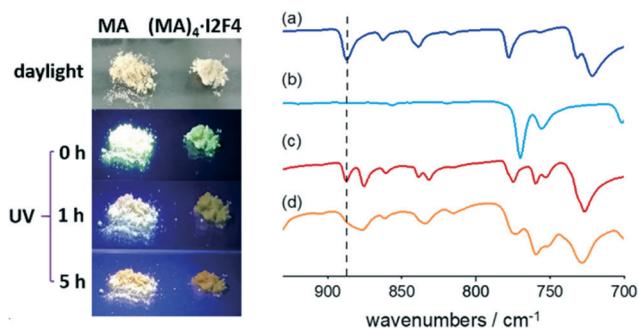
Fig. 4 Left: pictures taken during the UV irradiation of the polycrystalline samples of MA and (MA)_4\cdot I2F4 . Right: details of the FTIR spectra recorded on (a) crystalline MA, (b) the head-to-tail MA photodimer, (c) co-crystal (MA)_4\cdot I2F4 , and (d) the resulting amorphous solid after UV irradiation (right).
