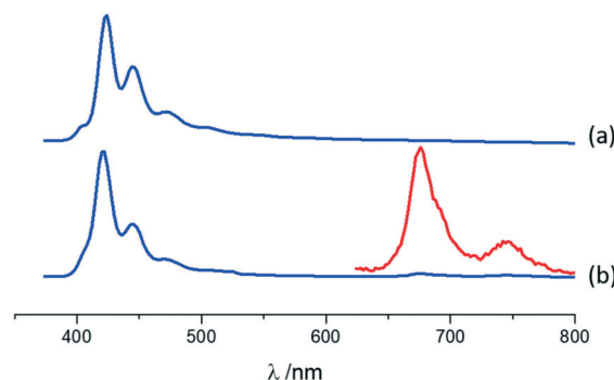
Fig. 5 Normalized luminescence spectra in the solid state for (a) pure A and (b) A\cdot(I2F4)_2 (arbitrary units on the y -axis). \lambda_{\text{exc}} = 380\text{ nm} . The phosphorescence spectrum in the 650–800 nm region, isolated with a gated detection, is magnified in the inset for A\cdot(I2F4)_2 . The phosphorescence emission is clearly evident in A\cdot(I2F4)_2 compared to solid anthracene, where no phosphorescence was detected.
