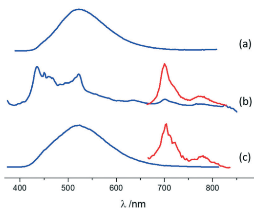
Fig. 6 Normalized luminescence spectra in the solid state of (a) pure MA, (b) MA\cdot I2F4 , and (c) (MA)_4\cdot I2F4 (arbitrary units on the y -axis). \lambda_{\text{exc}} = 380\text{ nm} . The phosphorescence spectra in the 650–850 nm region, isolated with a gated detection, are magnified in the inset for MA\cdot I2F4 and (MA)_4\cdot I2F4 . In both co-crystals the phosphorescence emission is clearly evidenced compared to the parent PAH 9-methylanthracene, where no phosphorescence was detected at all. Moreover, for MA\cdot I2F4 the spectrum is not dominated by excimer emission.
