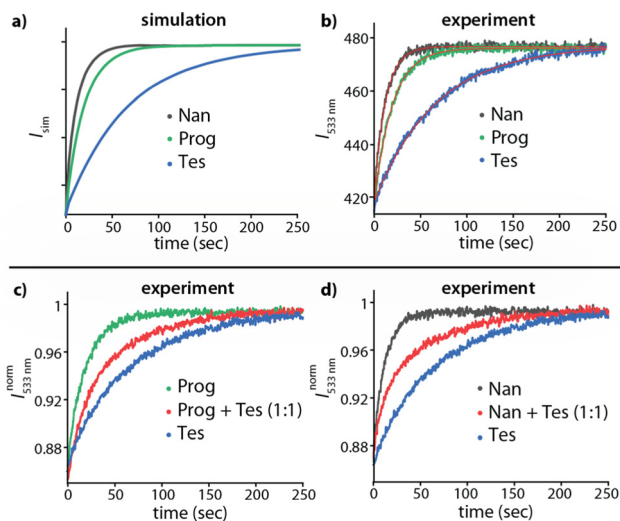
Fig. 4 (a) Simulated kinADA and (b) Experimental kinADA PFO traces monitored at 533 nm ( \lambda_{\text{exc}} = 376 nm) for CB8 \rightarrow Tes (1 \mu\text{M} , blue), CB8 \rightarrow Prog (1 \mu\text{M} , green) and CB8 \rightarrow Nan (1 \mu\text{M} , black) host \rightarrow analyte complex upon spiked addition of MPCP dye (50 \mu\text{M} ) in water. See Fig. S5 and S6 in the ESI† for further details and parameters used for the simulation. The red line in Fig. 4b depicts the fitted data according to the kinADA PFO binding model (eqn (1)). Experimental kinADA PFO traces monitored at 533 nm ( \lambda_{\text{exc}} = 376 nm) for a mixture of two steroids as analytes (red curve) in case of (c) CB8 (1 \mu\text{M} ), Tes (0.5 \mu\text{M} ) and Prog (0.5 \mu\text{M} ) and (d) CB8 (1 \mu\text{M} ), Tes (0.5 \mu\text{M} ) and Nan (0.5 \mu\text{M} ) upon spiked addition of MPCP (50 \mu\text{M} ) in water. The kinetic traces for individual steroids are shown for comparison.
