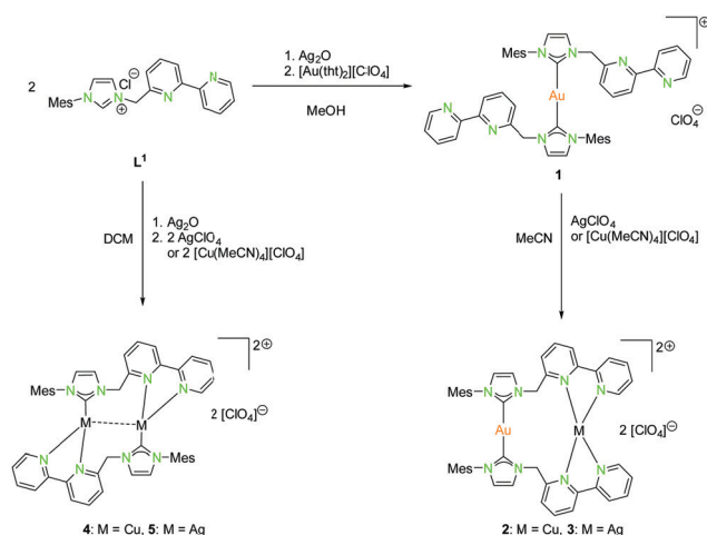
Scheme 1 Synthesis of mononuclear ( 1 ), dinuclear homo- ( 4 , 5 ) and heterobimetallic ( 2 , 3 ) compounds with NHC bipy ( L^1 ). 41
