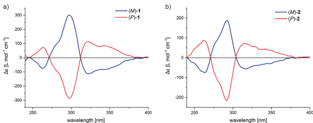
Fig. 6 Circular dichroism spectra of (a) ( P )-1 (red) and ( M )-1 (blue), (b) ( P )-2 (red) and ( M )-2 (blue) in CH 2 Cl 2 ( c ~ 10 -6 M). Absolute configuration was assigned according to exciton chirality method, DFT calculations and X-ray crystallography.
