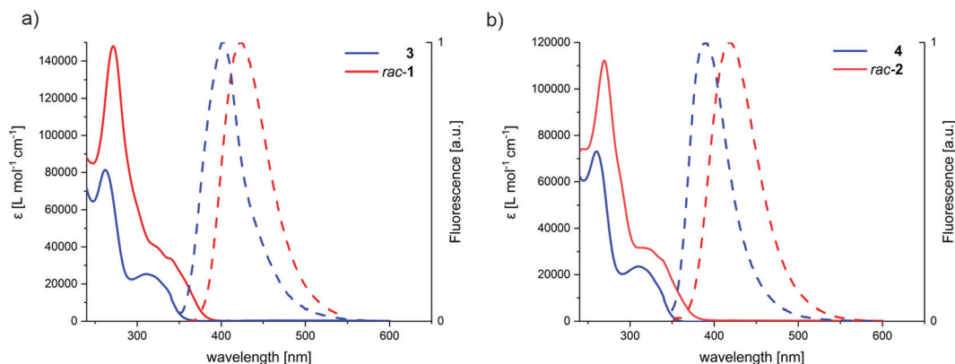
Fig. 5 Absorption (solid line) and emission (dashed line) spectra of (a) rac -1 (red) and its precursor 3 (blue), (b) rac -2 (red) and its precursor 4 (blue) in CH 2 Cl 2 ( c ~ 10 -6 M and 10 -7 M for absorption and emission, respectively). Compound 4 , 3 , rac -2 and rac -1 were excited at 313, 315, 322 and 340 nm, respectively.
