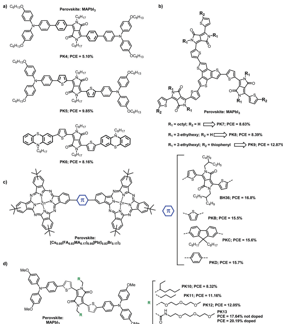
Fig. 22 (a) Chemical structures and PCEs for PK4–PK6 , (b) chemical structures and PCEs for PK7–PK9 , (c) chemical structures for BH36 , PKB , PKC and PKD , (d) chemical structures and PCEs for PK10–PK13 . Perovskite compositions are included.
