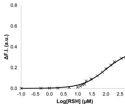
Fig. 7 Change in normalised fluorescence emission intensity at 440 \text{ nm} ( \lambda_{\text{exc}} = 365 \text{ nm} ) ( \Delta\text{F.I.} ) 360 \text{ min} after addition of different concentrations of benzyl thiol ( [\text{RSH}] ) to vesicles (DOPC, 1.0 \text{ mM} ) containing peptide substrate ( 250 \mu\text{M} ), caged papain ( 10 \mu\text{M} ) and 2 ( 10 \mu\text{M} , 1\% loading) in HEPES buffer (pH = 7.2). The line is the best fit to an isotherm for equilibrium formation of a 1 : 1 adduct between the thiol and 2 .
