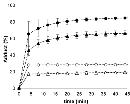
Fig. 5 Time course for conversion of 2 ( 50 \mu\text{M} ) embedded in vesicles (DOPC, 0.5 \text{ mM} in HEPES buffer at pH 7.2) into the corresponding Michael adduct on addition of different thiols: 100 \mu\text{M} benzyl thiol ( \blacktriangle ), 200 \mu\text{M} benzyl thiol ( \bullet ), 5.0 \text{ mM} 2-mercaptoethanesulfonate ( \triangle ), 10 \text{ mM} 2-mercaptoethanesulfonate ( \circ ).
