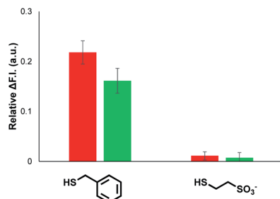
Fig. 6 Change in normalised fluorescence emission intensity at 440 \text{ nm} ( \lambda_{\text{exc}} = 365 \text{ nm} ) ( \Delta\text{F.I.} ) 360 \text{ min} after addition of two different thiols ( 100 \mu\text{M} ) to vesicles (DOPC, 1.0 \text{ mM} ) containing peptide substrate ( 250 \mu\text{M} ), caged papain ( 10 \mu\text{M} ) and either 1 (red) or 2 (green) at 1\% loading ( 10 \mu\text{M} ) in HEPES buffer (pH = 7.2).
