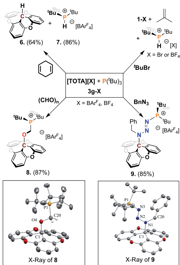
Scheme 3 FLPs mediated activation of small molecules. Unless otherwise noted all reactions were carried out on a 0.05 mmol scale using [\text{1}^+] , 0.05 mmol \text{P}(\text{t-Bu})_3 , 4 ml solvent, at room temperature. Isolated yields are given in parentheses ( \text{BARF}_4 = tetrakis(3,5-bis(trifluoromethyl)phenyl)borate). Crystal structures of 8 and 9 ; (thermal ellipsoids shown at 50% probability, hydrogen atoms and counter ion are omitted for clarity. P orange, N blue, C grey, O red).
