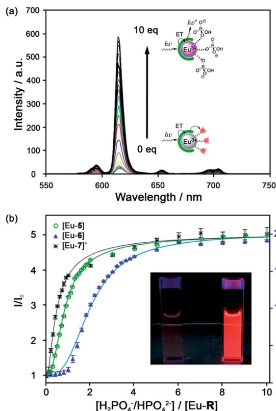
Fig. 6 (a) Increase in time-delayed (0.1 ms) luminescence of [Eu-6] upon titration with HPO 4 2- (H 2 O, pH 7.4); (b) luminescence titration data of [Eu-5], [Eu-6], and [Eu-7] + . Inset: Photo of [Eu-6] + solution in the absence and presence of 10 equiv. of HPO 4 2- . Reproduced from ref. 41 with permission from the American Chemical Society, copyright 2019.
