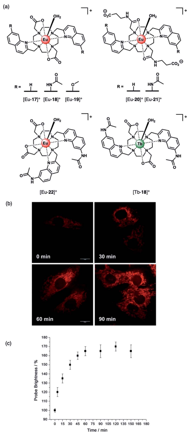
Fig. 8 (a) Family of cationic Eu(III) and Tb(III) complexes capable of discriminating between nucleoside tri-, di- and monophosphate anions (e.g. ATP, ADP and AMP); (b) Real-time monitoring of elevated ATP levels in the mitochondria of living cells. Time-lapsed LSCM images of NIH-3T3 cells stained with [Eu-21] + (50 \mu M, \lambda_{\text{exc}} 355 nm, \lambda_{\text{em}} 605–720 nm) before (0 min) and after treatment with staurosporine (10 nM), a potent inhibitor of protein kinases; (c) time-dependent increase in emission intensity (605–720 nm) of cells stained with [Eu-21] + following treatment with staurosporine (10 nM). Reproduced from ref. 58 with permission from Wiley-VCH, copyright 2018.
