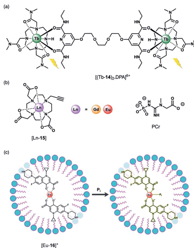
Fig. 7 (a) Tb(III)-Based displacement assay for HPO 4 2- and NO 3 - ; (b) alkyne-functionalised DO3A complex for assessing bulk phosphate species (PCr, HPO 4 2- ); (c) schematic depiction of the detection of HPO 4 2- (Pi) in water samples, using a Eu(III)-CIP mixture in the presence of the surfactant SDBS.
