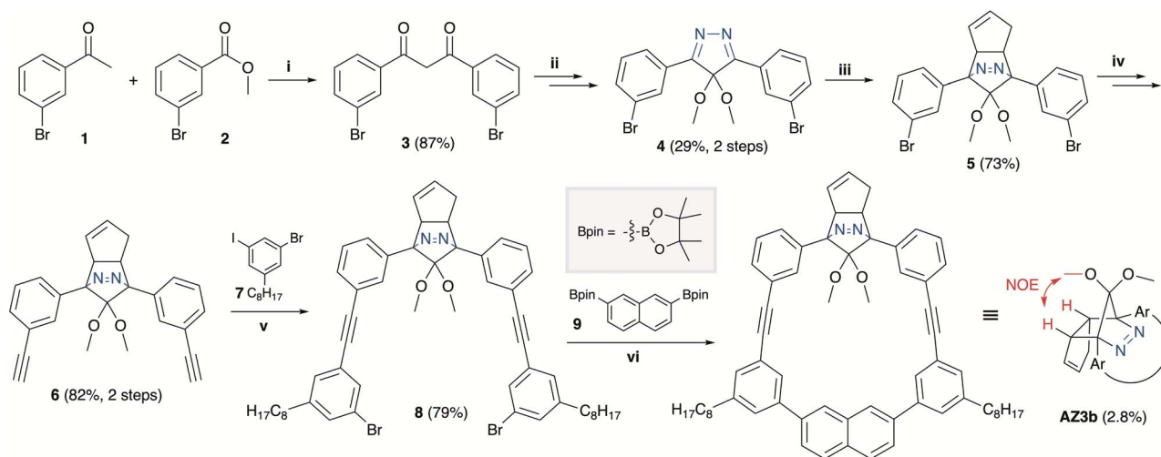
Scheme 3 Synthetic route towards AZ3b . (i) NaH, THF, 0 °C, 20 h; (ii) 1 , Ph 2 Se 2 , (NH 4 ) 2 S 2 O 8 , MeOH, 75 °C, 3.5 h; 2 , (NH 4 ) 2 S 2 O 8 , MeOH, 75 °C, 3.5 h; (iii) N 2 H 4 ·H 2 O, CHCl 3 , 70 °C, 16 h; (iv) cyclopentadiene, TFA, DCM, 0 °C, 1.5 h; (v) trimethylsilylacetylene, Pd(PPh 3 ) 4 , CuI, TEA, THF, 60 °C, 43.5 h; 2 , K 2 CO 3 , THF, MeOH, r.t., 16.5 h; (vi) Pd(PPh 3 ) 4 , CuI, TEA, THF, 60 °C, 39.5 h; (vii) Pd(OAc) 2 , SPhos, K 3 PO 4 , THF, H 2 O, 80 °C, 21 h.
