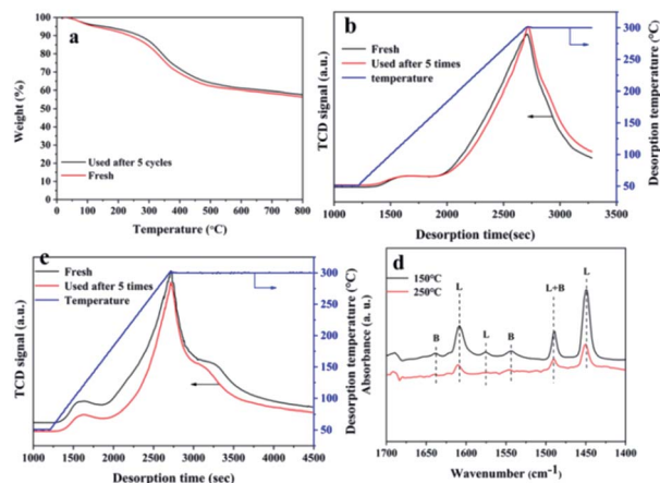
Fig. 9 Characterization of acid–base sites of catalysts before and after recycling: (a) TG curves, (b) \text{CO}_2 -TPD curves, (c) \text{NH}_3 -TPD curves, (d) pyridine-adsorbed FT-IR spectra (L: Lewis acid, B: Brønsted acid).
