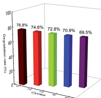
Fig. 8 Recycled experiments of the \text{E-Bi}_2\text{O}_2\text{CO}_3 photocatalyst.
