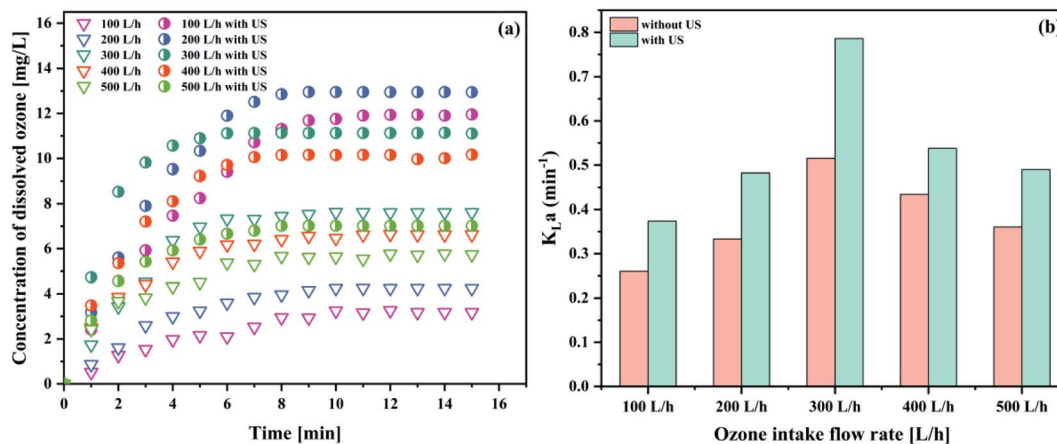
Fig. 6 Effect of the intake flow rate on (a) the concentration of dissolved ozone and (b) K_La (pH 3; gaseous ozone concentration 32.38 mg L -1 ; temperature 293.15 K; US power 1000 W).
