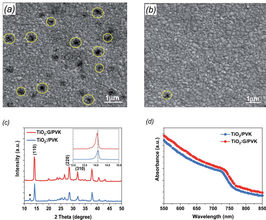
Fig. 3 (a) FESEM image of perovskite deposited on a pure \text{TiO}_2 layer. (b) Perovskite on a G:TiO 2 layer. (c) XRD patterns of perovskites. The asterisk indicates the reflection of \text{PbI}_2 . Inset: zoomed-in view of the peak at 14° of the perovskites. (d) Absorption spectra of perovskite films deposited on pure and modified \text{TiO}_2 layers.
