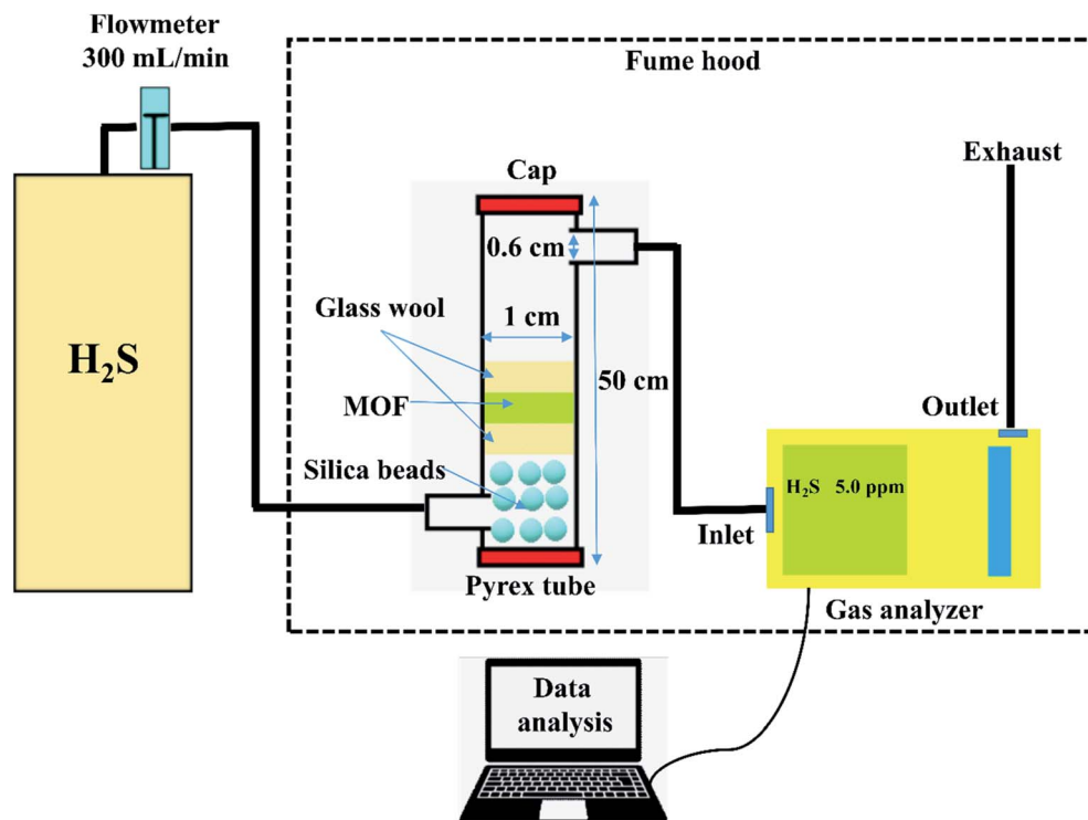
Fig. 1 Schematic illustration of the H 2 S adsorption system.
