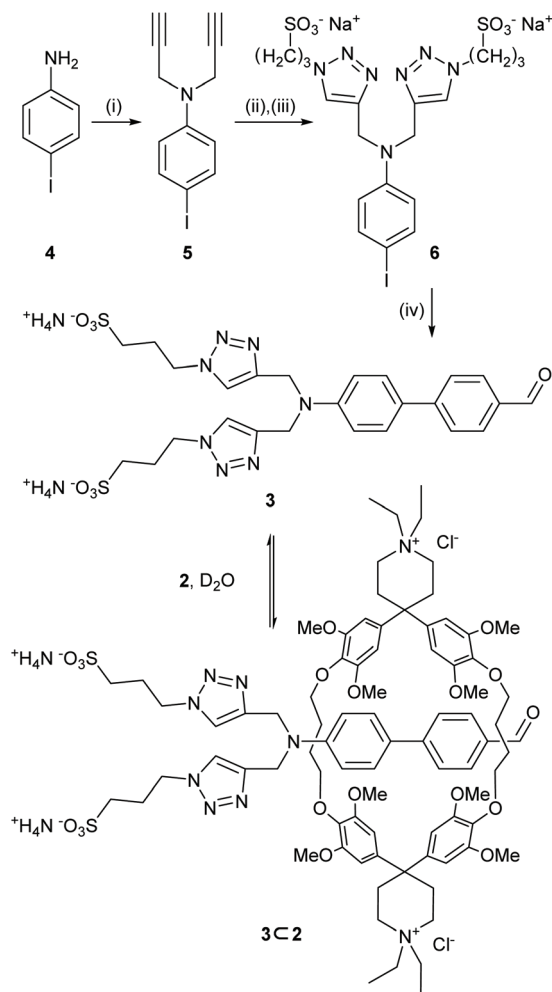
Scheme 2 Synthesis of 3 and pseudorotaxane formation with 2 in D_2O . (i) Propargyl bromide (30 wt% in toluene), K_2CO_3 , ACN, 60^\circ C , 3 d, 66%; (ii) NaN_3 , 1,3-propanesultone, DMF/ H_2O (2:1), rt, 1 h; (iii) TBTA, Cu (CH_3CN)_4PF_6 , sodium ascorbate, 5 , rt, 22 h, 45%; (iv) 4-formylphenylboronic acid, K_3PO_4 , Pd(OAc)_2 , H_2O , reflux, 1 h, 78%.
