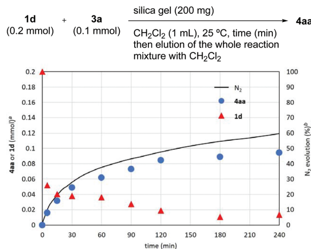
Fig. 1 Time course studies of the reaction of 1d and 3a . a Determined by 1 H NMR spectroscopy using 1,1,2,2-tetrachloroethane as an internal standard. b Based on 1d (0.8 mmol).
