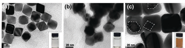
Fig. 3 TEM images of (a) Pd Octas, and samples obtained (b) without and (c) with CTAB. Insets correspond to the digital photos of the final solutions after preparation.
