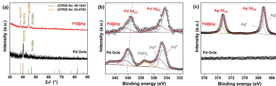
Fig. 2 (a) XRD patterns and XPS profiles of (b) Pd 3d and (c) Ag 3d of Pd@Ag cubes and Pd Octas.
