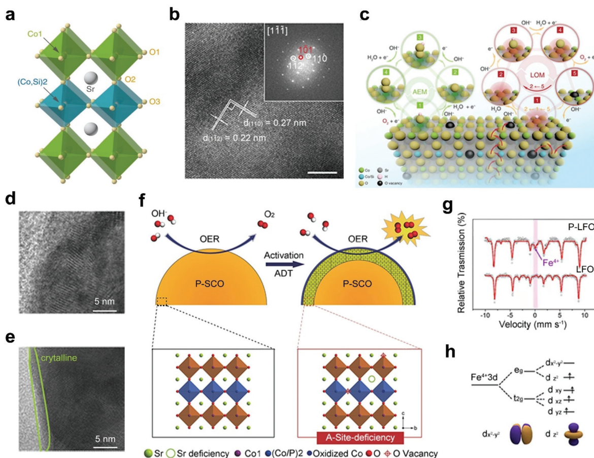
Fig. 7 (a) Schematic representation of the crystal structure of Si-SiO x -SCO. (b) HRTEM image of Si-SiO x -SCO and the corresponding FFT pattern. (c) Schematic representation of the AEM and LOM reaction pathways on Si-SiO x -SCO. Reproduced with permission from ref. 58. Copyright 2020, Nature Publishing Group. (d) HRTEM images of surface regions of P-SCO (d) before and (e) after 1000 cycles. (f) Schematic representation of the main origin of the OER activation in the SCP sample. Reproduced with permission from ref. 57. Copyright 2016, Wiley-VCH. (g) Mössbauer spectrum of the main origin of the OER activation in the SCP sample. Reproduced with permission from ref. 57. Copyright 2016, Wiley-VCH. (h) Schematic representation of Fe 3d orbit degeneration. Reproduced with permission from ref. 87. Copyright 2018, Elsevier B.V.
