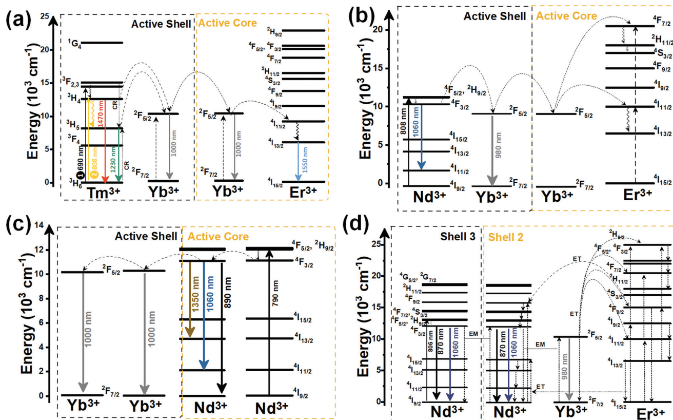
Fig. 27 (a) Mechanisms of generation of the emission lines of core@shell nanostructures: (a) \text{Er}^{3+}, \text{Yb}^{3+}:\text{LaF}_3@ \text{Tm}^{3+}, \text{Yb}^{3+}:\text{LaF}_3 nanocrystals excited either at 690 nm or 808 nm, (b) \text{Er}^{3+}, \text{Yb}^{3+}:\text{NaYF}_4@ \text{Nd}^{3+}, \text{Yb}^{3+}:\text{NaYF}_4 nanoparticles excited at 808 nm, (c) \text{Nd}^{3+}:\text{LaF}_3@ \text{Yb}^{3+}:\text{LaF}_3 nanoparticles excited at 790 nm, and (d) \text{Tm}^{3+}, \text{Yb}^{3+}:\text{SrF}_2@ \text{Y}^{3+}:\text{SrF}_2@ \text{Er}^{3+}, \text{Nd}^{3+}, \text{Yb}^{3+}:\text{SrF}_2@ \text{Nd}^{3+}:\text{SrF}_2 nanocrystals excited at 806 nm.
