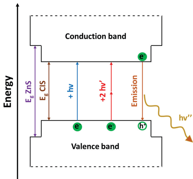
Fig. 7 Schematic representation of the non-resonant two-photon excitation process (red arrows) and two-photon excited luminescence (orange arrow) in colloidal quantum confined CuInS 2 /ZnS type-I core/shell heterostructures, compared to the classical absorption mediated by one photon (blue arrow). Here, h\nu > h\nu' .
