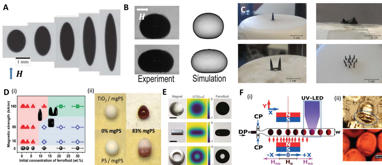
Fig. 8 Magnetic method for manipulating microdroplets. (A) Elongated PDMS ferrofluid droplet emerging in glycerol solution under various magnetic field strengths ( H = 6.0, 12.2, 23.9, 59.8, 162.3 kA m -1 (from left to right)). (B) Experimental and numerical results of the deformation of a sessile ferrofluid droplet under the different magnetic field strengths ( B_{0m} = 57 for top and 807 for bottom). (C) Magnetically triggered ferrofluid droplet deformation and division on a superhydrophobic surface when the magnetic field intensity increases. (D) (i) Structure map of the supraparticles with various shapes obtained by the evaporation-guided assembly of magnetic nanoparticles. (ii) Binary supraparticles fabricated by drying a co-suspension under magnetic field. (E) Complex shapes of ferrofluid droplet produced by permanent magnets in disk-, cube-, and ring-shapes; the scale bar is 10 mm. (F) (i) Synthesis of magnetic Janus particles within a flow focusing droplet generation system with magnetic field and UV LED. (ii) Optical images of generated magnetic Janus particles. The blue ellipse indicates the accumulated magnetic components. Reproduced with permission from ref. 124, 128, 131–133 and 138. Copyright 2010 and 2018 Cambridge University press. Copyright 2011 and 2017 Royal Society of Chemistry. Copyright 2019 American Chemical Society. Copyright 2010 National Academy of Sciences.
