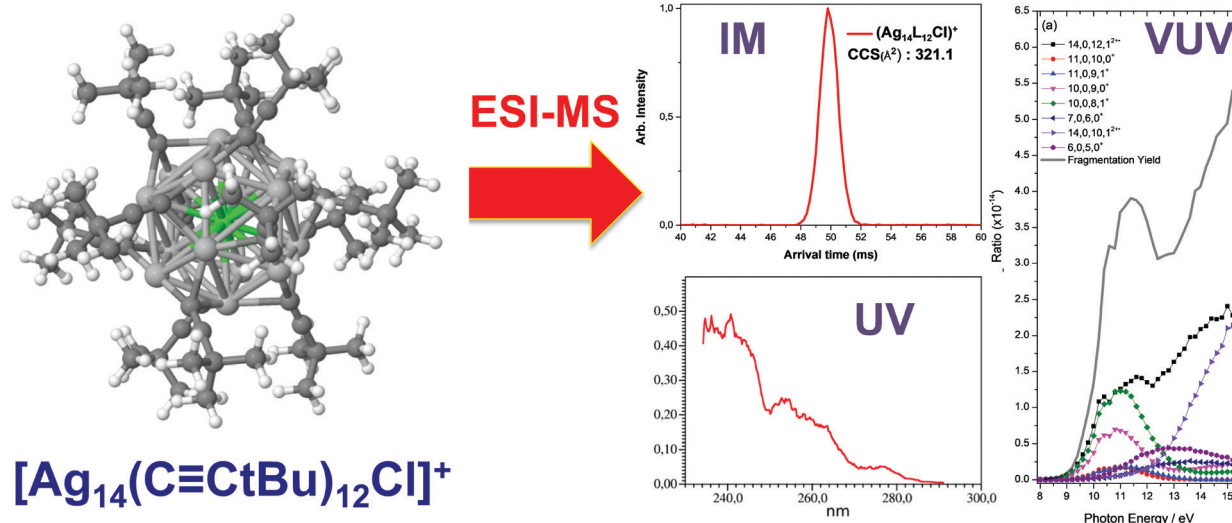
Fig. 11 DFT-optimized structures (chlorine, light green; silver, light gray; copper, orange; carbon, dark green; hydrogen, white) for [Ag_{14}(C\equiv CtBu)_{12}Cl]^+ with ion-mobility arrival times (red peak) and optical action spectra in the UV and VUV range. (reprinted with permission Copyright © 2017 American Chemistry Society). 203
