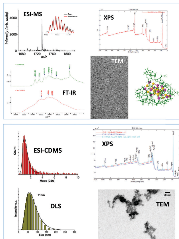
Fig. 12 Examples of characterization techniques in addition to mass spectrometry used for atomically precise Au_{15}SG_{13} nanoclusters (top panel) and sub-100 nanometer silver doped gold–cysteine supramolecular assemblies (bottom panel). XPS: X-ray photoelectron spectroscopy, FT-IR: Fourier-transform IR spectroscopy, TEM: Transmission electron microscopy, DLS: dynamic light scattering.
