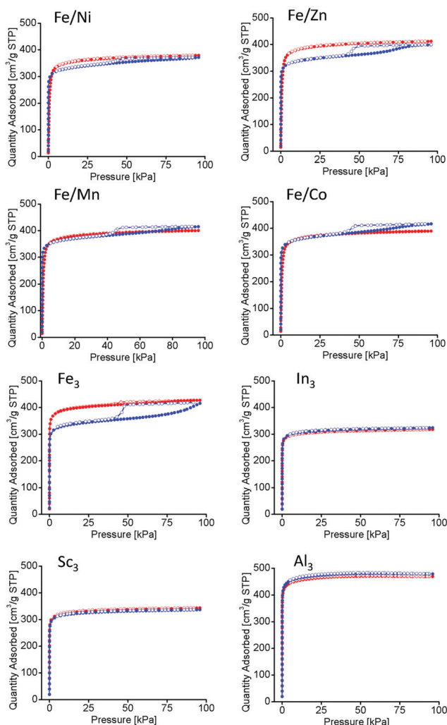
Fig. 5 Nitrogen Isotherms at 77 K before (red) and after (blue) 100 hour thermal activation. In the Fe/Ni, Fe/Zn, Fe/Mn, Fe/Co, Fe 3 , clusters a hysteresis loop is observable indicating mesopore formation. Samples for In 3 , Sc 3 , and Al 3 do not have mesopore formation.
