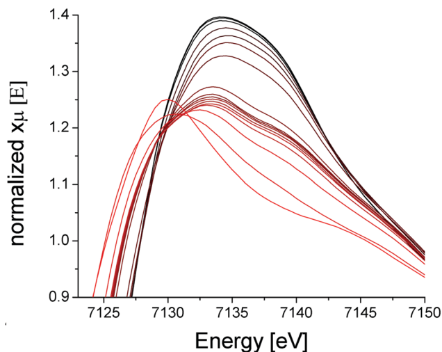
Fig. 4 XAS spectra of PCN-250 (Fe 3 ) in the range of 23 °C (black) to 450 °C (red).
