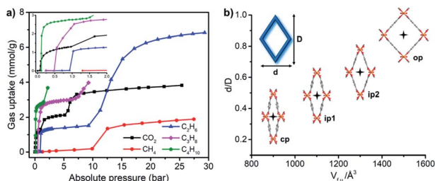
Fig. 7 (a) Gas sorption isotherms recorded for MIL-53(Fe) at 303 K; (b) different phases observed in MIL-53(Fe), cp = closed phase, ip = intermediate phase, op = open phase.
