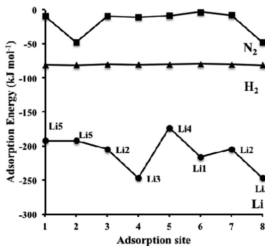
Fig. 8 Dispersion-corrected (revPBE-D3) adsorption energies of Li (circles), H_2 (triangles) and N_2 (squares) over the symmetry unique adsorption sites on \eta\text{-Mn}_3\text{N}_2 depicted in Scheme 1 (for H_2 and N_2 ). The data for Li corresponds to the adsorption site configuration depicted in Scheme 2. Lines connecting the data points have been drawn to guide the eye.
