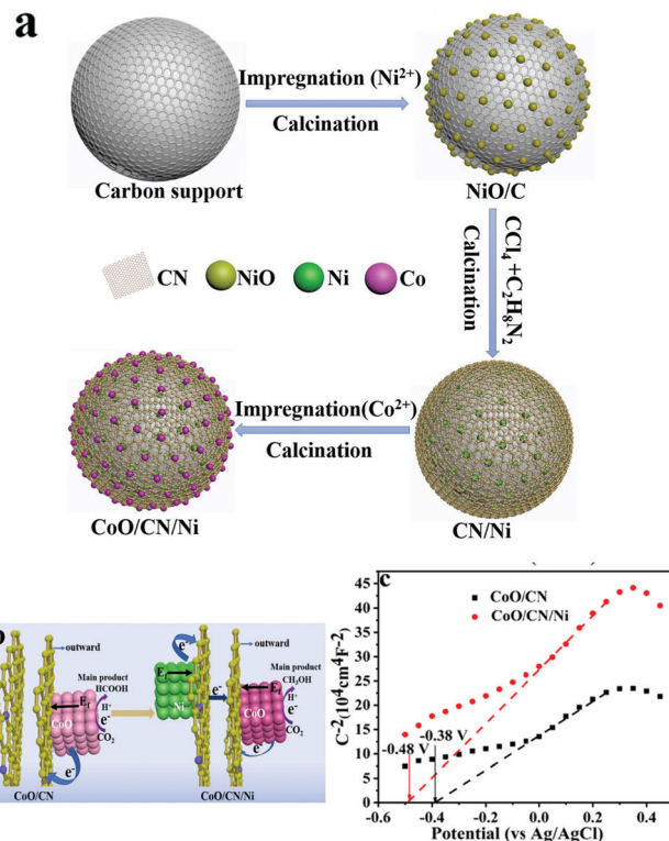
Fig. 8 (a) Sketch of the synthetic sequence for the assembly of the ternary CoO/CN/Ni catalyst; (b) graphical representation of the factors controlling product selectivity in CO 2 RR by the binary and ternary catalysts; (c) Mott-Schottky analysis of the ternary hybrid and of the Ni-free binary catalyst. Reprinted from ref. 56, (2021) with permission from Elsevier.
