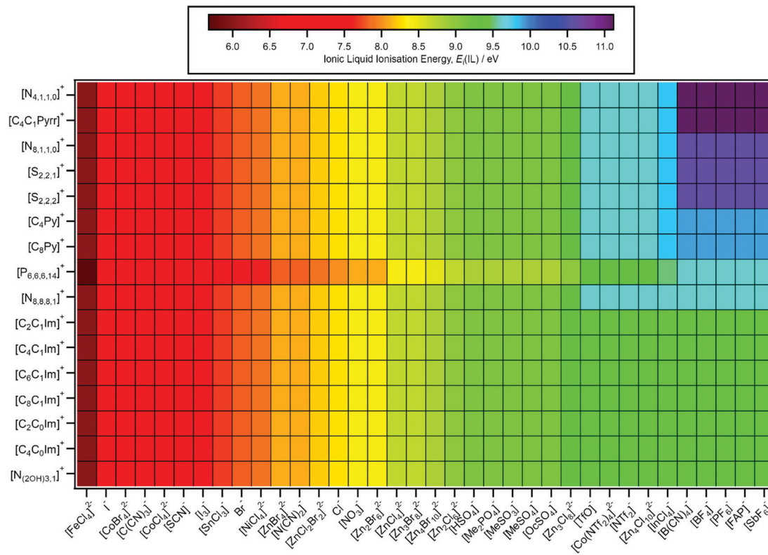
Fig. 6 Predicted IL ionisation energies, E_i(\text{IL, pred.}) . The errors in E_i(\text{IL, pred.}) generally range from \pm 0.2 eV to \pm 0.4 eV.
