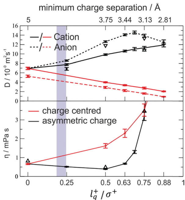
Fig. 16 Diffusion and viscosity as a function of charge separation. The blue shaded area indicates the l_q^+/\sigma^+ range for the [\text{C}_4\text{C}_{1}\text{im}] cation. The charge centred systems where charge separation is achieved by decreasing the size are shown in red. Reprinted (adapted) from H. V. Spohr and G. N. Patey, J. Chem. Phys. , 2009, 130 , 104506, with the permission of AIP Publishing. 217
