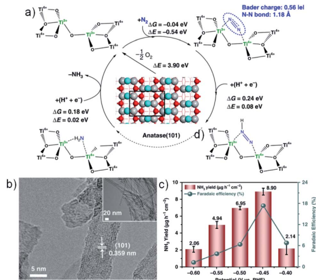
Fig. 5 (a) DFT prediction of the NRR activity for adjacent bi-Ti 3+ on anatase (101) with V O (light-blue spheres: lattice oxygen at the bridge sites where the surface V O are formed most easily; red spheres: other lattice oxygens on the surfaces; gray spheres: titanium cations; \Delta G : free energy; \Delta E : electronic energy. (b) TEM image for Zr-TiO 2 nanotubes. (c) \text{NH}_3 yields and FEs of Zr-TiO 2 at each given potential. Reproduced from ref. 88 with permission from the Nature Publishing Group, copyright 2019.
