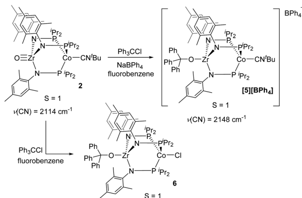
Scheme 2 The reactivity of 2 with \text{Ph}_3\text{C}^+ reagents.
