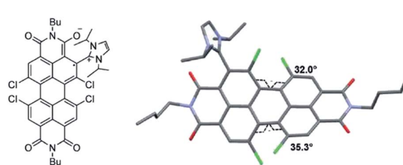
Fig. 4 Imidazolium cation stabilized PBI radical anion and its single crystal structure. Reproduced from ref. 45 with permission from Wiley-VCH, Copyright 2015.
