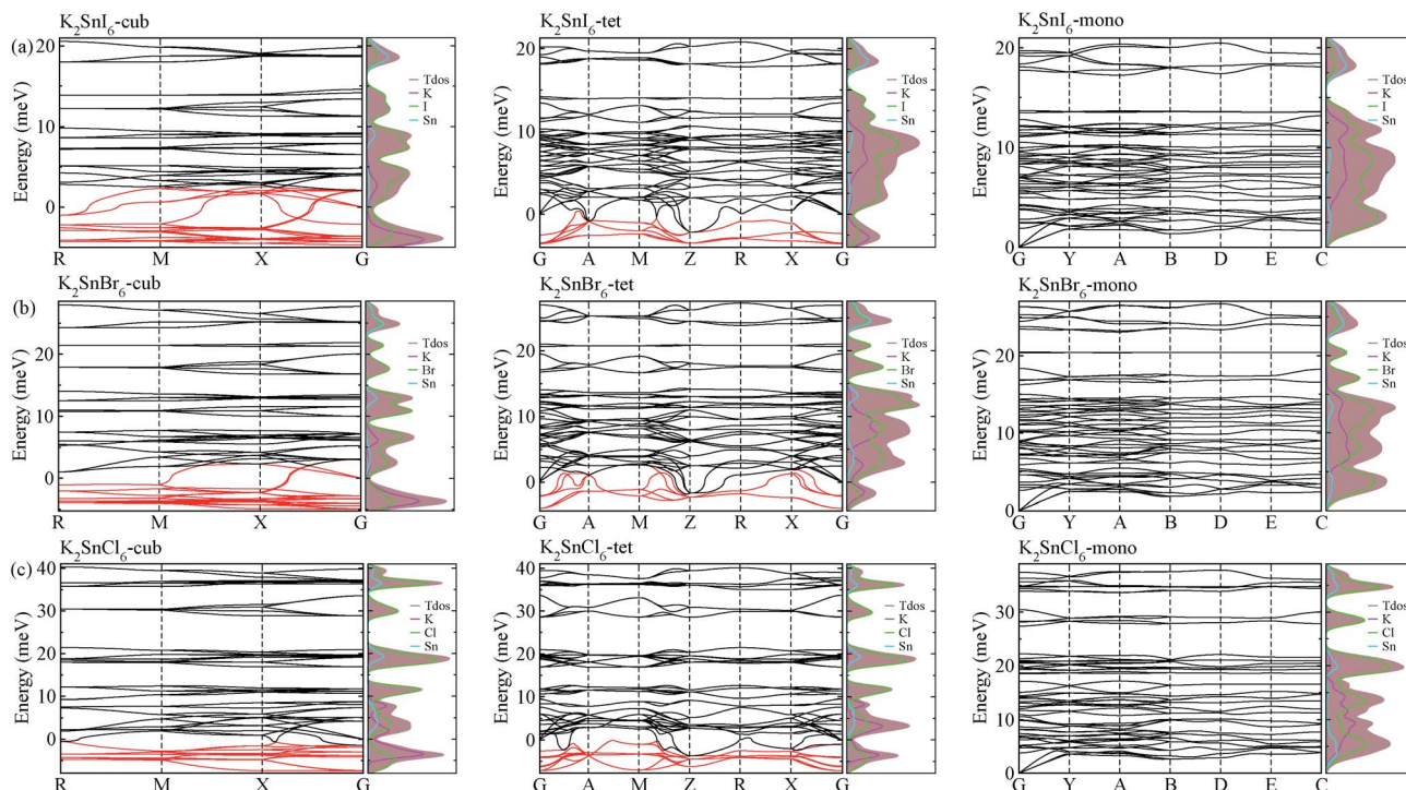
Fig. 4 Phonon dispersion curves and atomic resolved density of states in (a) \text{K}_2\text{SnI}_6 , (b) \text{K}_2\text{SnBr}_6 and (c) \text{K}_2\text{SnCl}_6 in the cubic (left), tetragonal (middle) and monoclinic (right) phases. Red lines show the anharmonic phonon modes with negative phonon energies.
