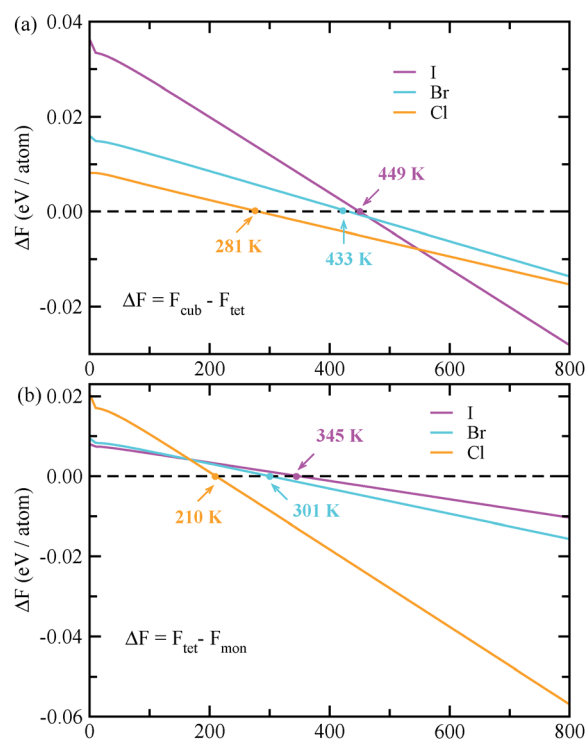
Fig. 5 Helmholtz free energy differences between (a) cubic and tetragonal phases, and (b) tetragonal and monoclinic phases in \text{K}_2\text{SnX}_6 ( X = \text{I}, \text{Br}, \text{Cl} ).
