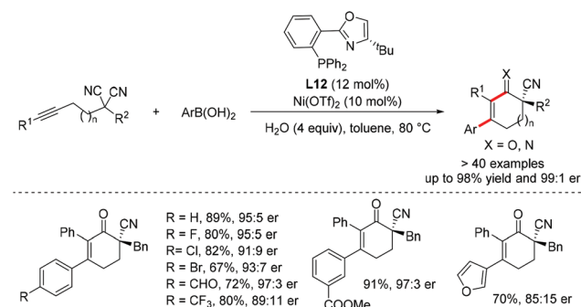
Scheme 33 Ni-Catalyzed cyclization of alkynyl electrophiles with organoboronic acids involving anti -carbonickelation of alkynes.
