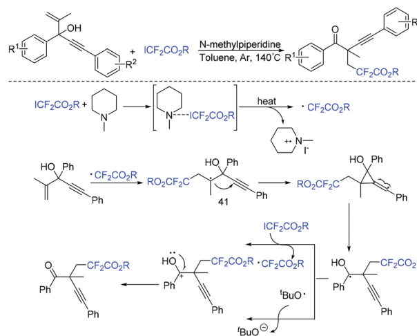
Scheme 20 The base-promoted difluoroalkylation reaction of 1,4-enynes with \text{ICF}_2\text{CO}_2\text{Et} .
