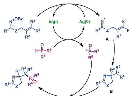
Scheme 20 Proposed mechanism.
