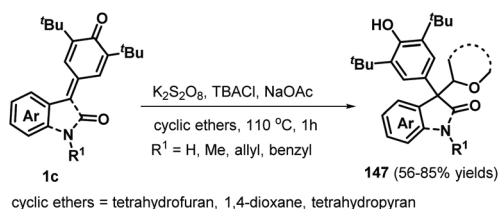
Scheme 30 Radical 1,6-addition of cyclic ethers to p -QMs.
