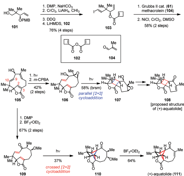
Scheme 16 Biomimetic transannular [2 + 2] photocycloaddition in the total synthesis of (+)-aquatulide.
