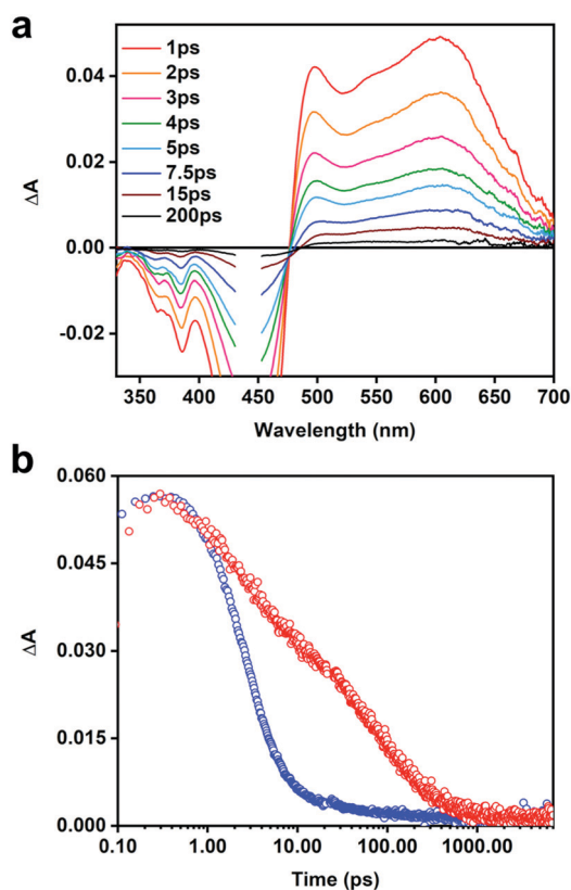
Fig. 5 (a) Picosecond TA spectra of CPE (12.5 \mu\text{M} , PRU) + 12.5 \mu\text{M} NDI 2+ in air-saturated \text{H}_2\text{O} at the indicated delay times following a 440 nm laser excitation pulse (100 fs pulse width, 100 nJ per pulse). (b) Kinetic decay traces of CPE (red) and CPE + NDI 2+ (blue) detected at 603 nm and 622 nm, respectively.
