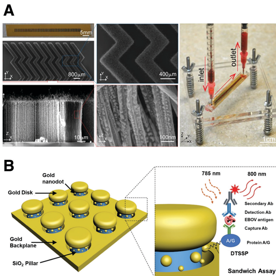
Fig. 5 Biosafety materials for virus capture and detection. (A) High-throughput microfluidic VIRRIION platform containing carbon nanotube arrays for influenza virus capture and identification. Reproduced with permission from ref. 104. Copyright 2020, National Academy of Sciences. (B) Schematic illustration of 3D plasmonic nanoantenna array for EBOV sensor. Reproduced with permission from ref. 106. Copyright 2019, Wiley-VCH.
