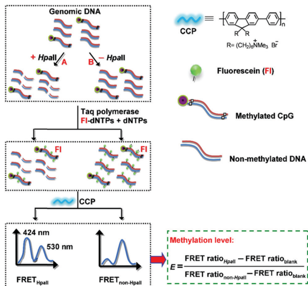
Fig. 46 Schematic illustration of the CCP-based FRET technique for DNA methylation detection. The methylation level ( E ) of DNA is calculated according to FRET ratios ( I_{530\text{ nm}}/I_{424\text{ nm}} ) of HpaII-treated, untreated, and blank control samples. Reprinted from ref. 288 with permission. Copyright (2012) from Nature Publishing Group.
