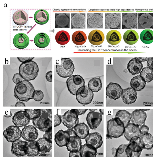
Fig. 15 (a) Schematic illustration of the preparation of triple-shelled NiO, \text{Co}_3\text{O}_4 , and their mixed oxide (Ni–Co–O) hollow spheres. (b–g) Typical TEM images of these samples. Reprinted from ref. 60 with kind permission.
