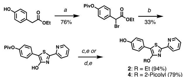
Scheme 1 Synthesis of HPPT derivatives 2 and 4. (a) (i) PivCl, DMAP, pyridine; (ii) NBS, AIBN, TBT, 80 °C. (b) 2-Pyridylthioamide, EtOH, 90 °C (μW). (c) EtI, K 2 CO 3 , acetone. (d) 2-PicBr-HBr, K 2 CO 3 , acetone. (e) K 2 CO 3 , MeOH. See ESI† for reagent abbreviations.
