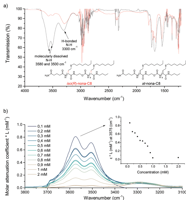
Fig. 6 (a) Comparison of IR-absorption iso(R) -nona-C8 and at -nona-C8, whereby two different N - H stretches are indicated. (b) Molar attenuation coefficient of iso(R) -nona-C8 at different concentration and at 3575 cm -1 .
