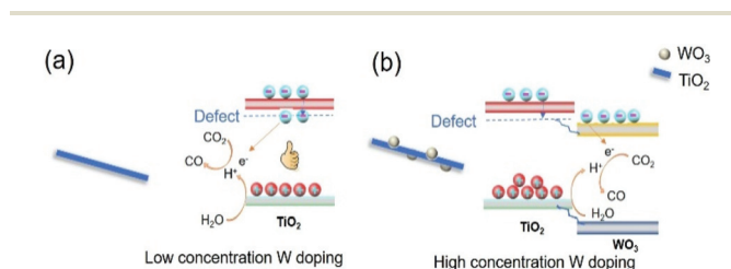
Fig. 8 Scheme of W-doped \text{TiO}_2 over different doping concentration, (a) low concentration and (b) high concentration.
