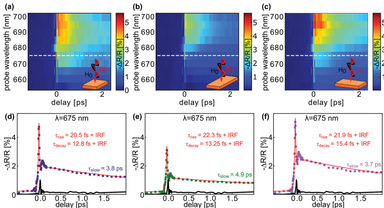
Fig. 5 Differential reflectivity -\Delta R/R contour plots with respect to the probe wavelength and the pump-probe delay time for three patches with dimensions (a) 625 nm × 625 nm, (b) 625 nm × 850 and (c) 850 nm × 625 nm. The dashed lines mark the 675 nm probe wavelength that is shown in temporal traces (d)–(f) for the respective patches. Red solid lines represent fittings to the convolution of exponential rise/decay and the IRF for the ultrafast response and exponential decay for the slow decaying part, respectively. The resulting time constants are indicated. The response of the as-deposited a-GaP film is shown in black.
