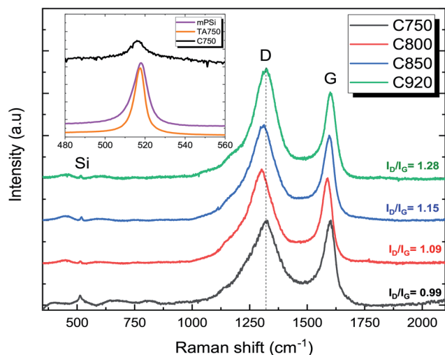
Fig. 3 Raman spectra of GPSi-nCs presents D and G bands characteristic of graphene. Spectra are vertically shifted for clarity. The inset in the figure illustrates the Si band for mPSi, TA750 and C750 samples.
