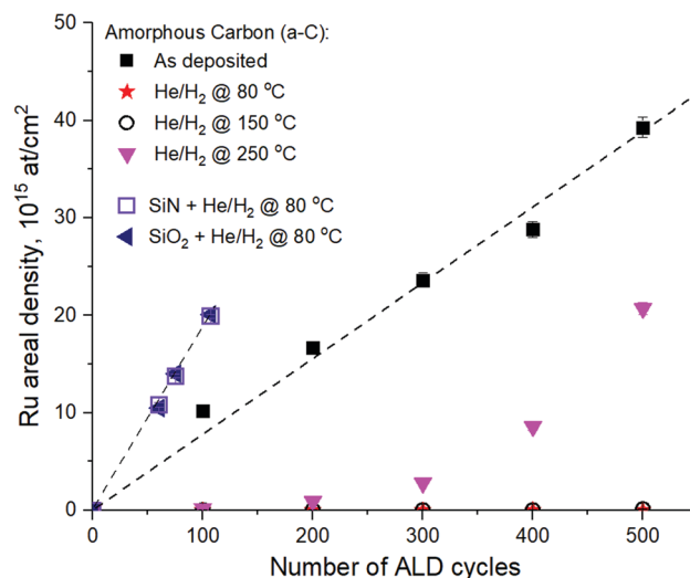
Fig. 4 RBS areal density of Ru as a function of ALD cycle number.
