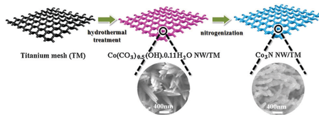
Fig. 14 Schematic diagram of Co 3 N NW/TM synthesis. Reproduced ref. 180 with permission from Elsevier B.V., copyright 2017.
