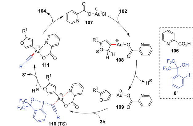
Scheme 17 \pi -Activation mode and interplay mode of Au-catalysis giving rise to regioselective approaches towards C2- and C3-alkynyl furans, respectively.
